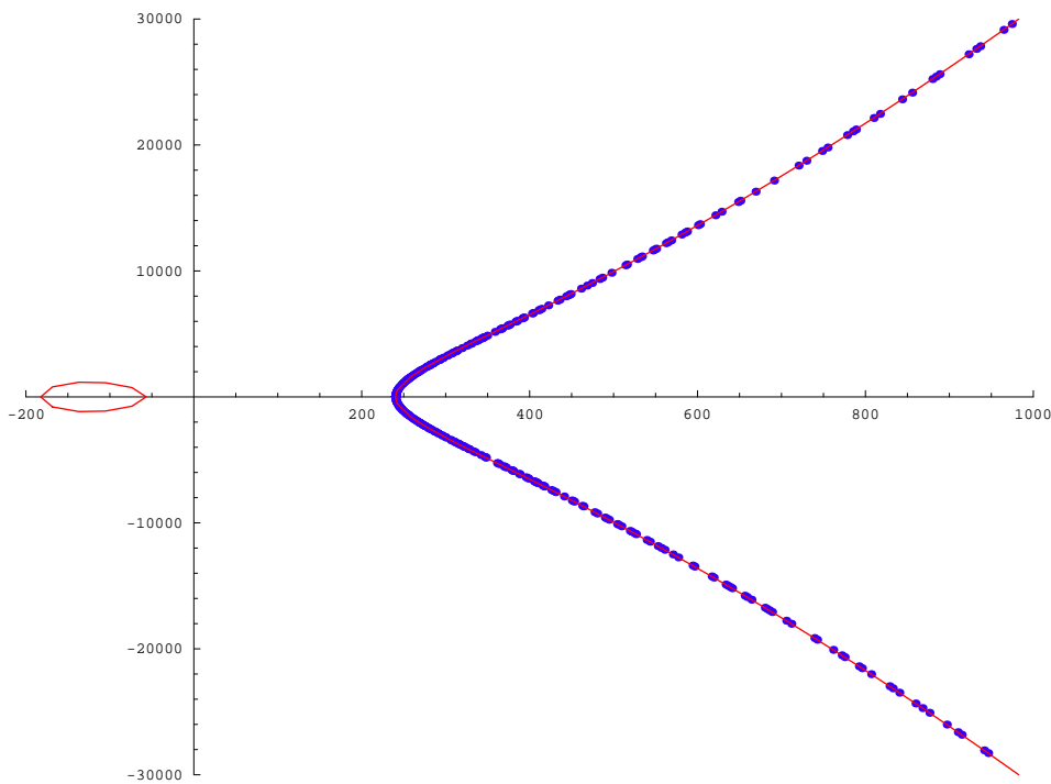
Figure 3: nP_2 , 1 \leq n \leq 1000 in blue , and E(\mathbb{R}) in red
